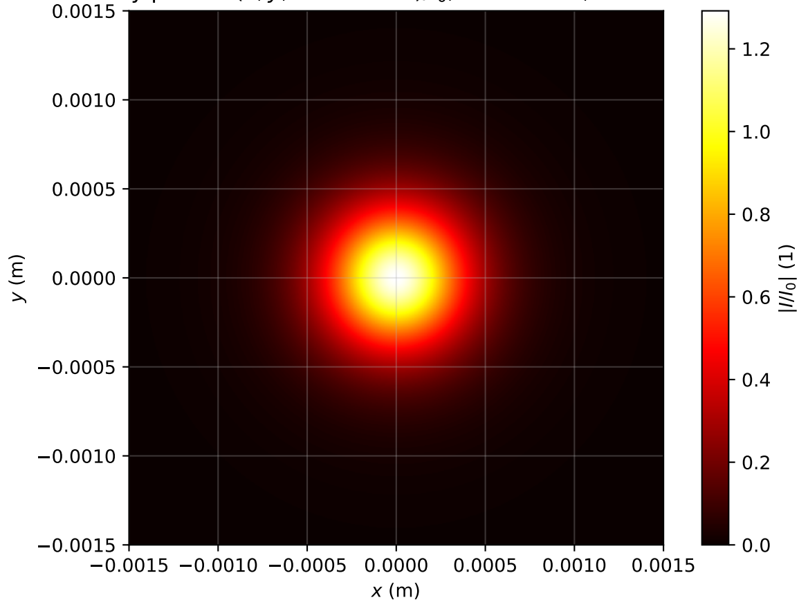
Intensity profile I(x, y, z = 2.149m)/I_0 , Pin=0.8Pcr, artificial time
